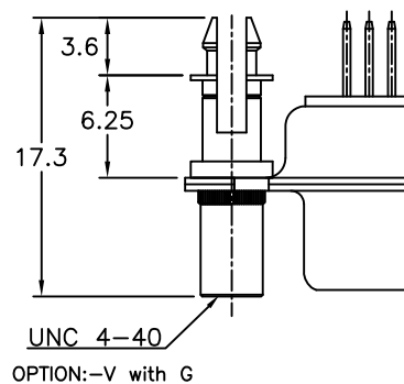
HARPOON PRESS FITTED TO SHELL
