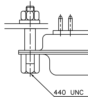
EXTENDED FEMALE SCREW LOCK WITH SPACER
