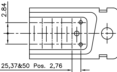
LAY OUT OF 50P CONNECTOR
