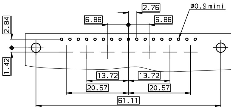
LAYOUT DIMENSIONS (after plating) CONNECTOR SIDE VIEW
