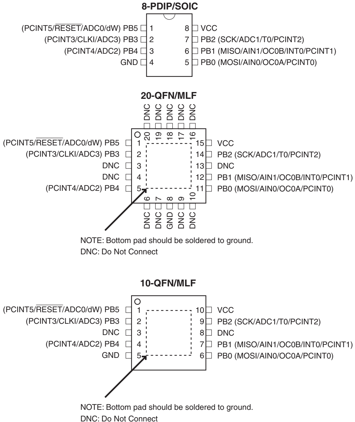
Figure 1-1. Pinout ATtiny13/ATtiny13V
