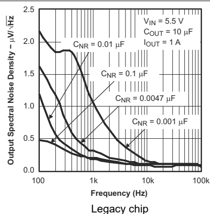
Figure 5-10. TPS79630 Output Spectral Noise Density vs Frequency
