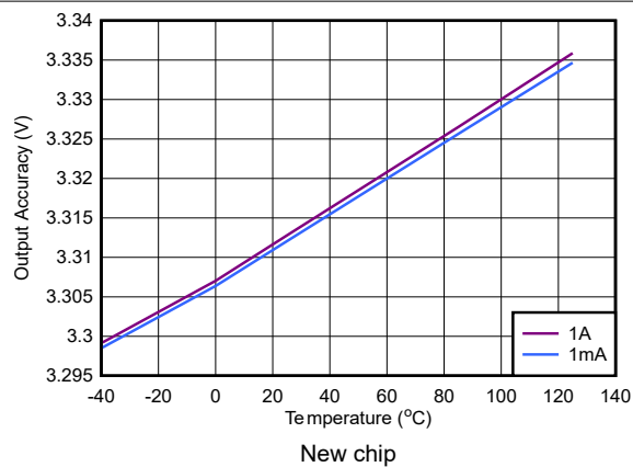
Figure 5-4. TPS79633 Output Voltage vs Junction Temperature
