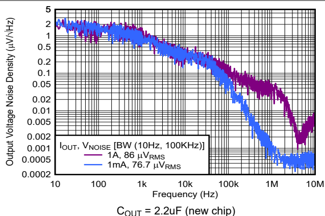
Figure 5-8. TPS79633 Output Spectral Noise Density vs Frequency
