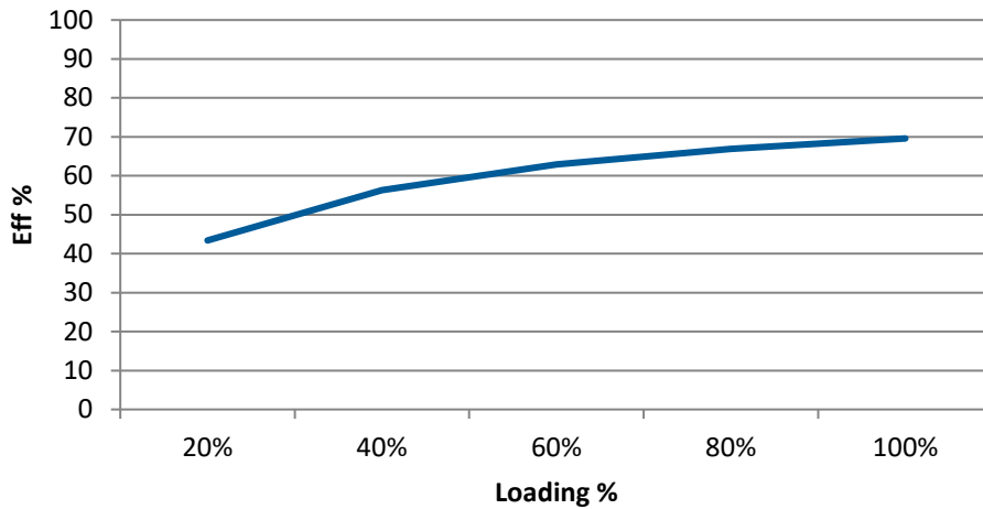
AM2F-1212SZ Efficiency vs. Loading
