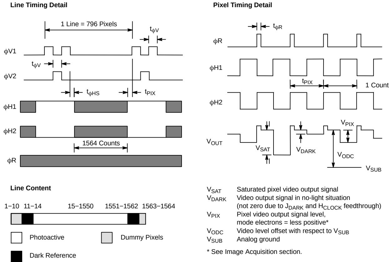
Figure 10. Timing Diagrams
