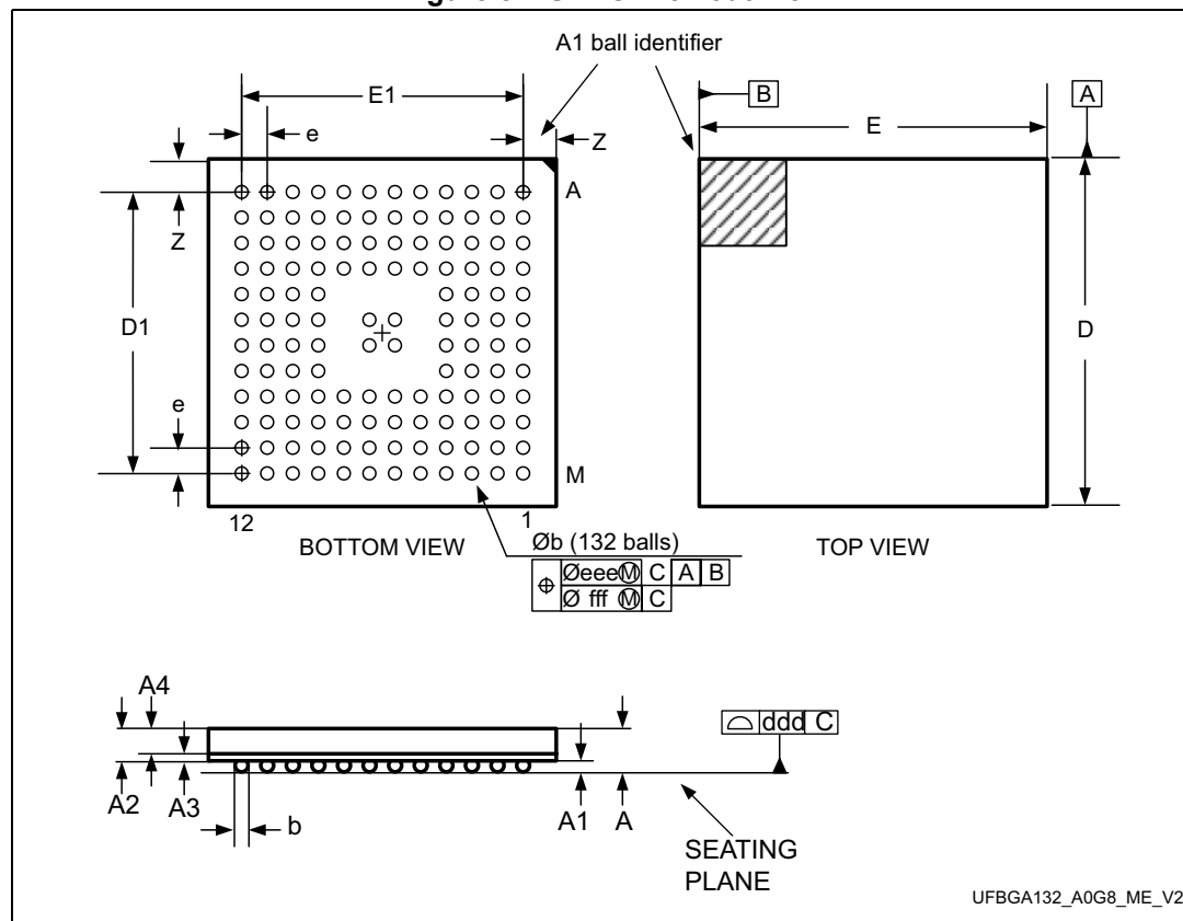
Figure 87. UFBGA132 outline
