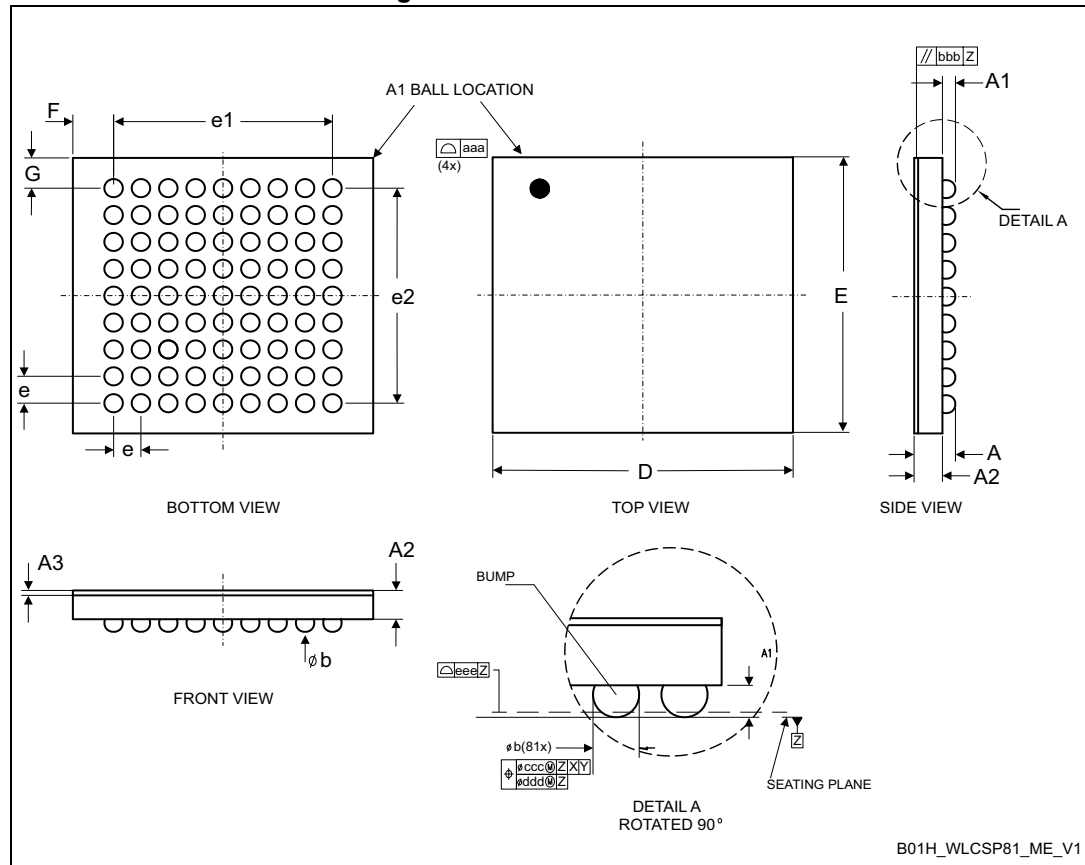
Figure 82. WLCSP81 outline
