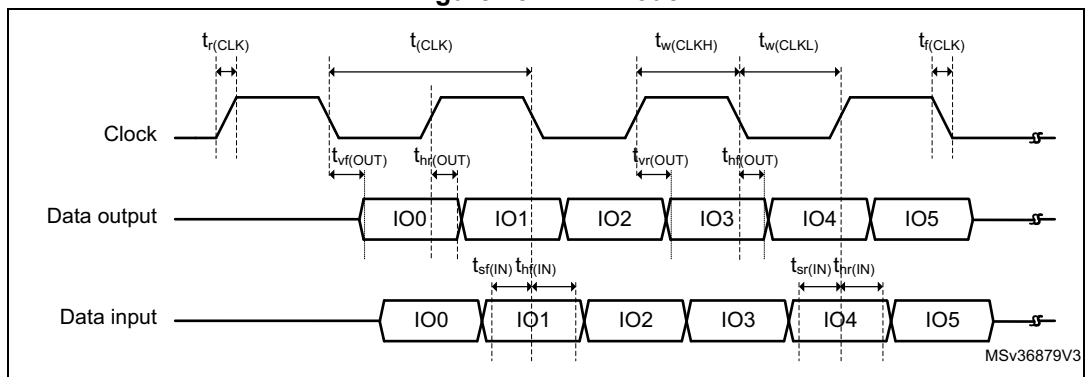
Figure 75. DDR mode
