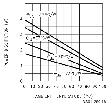
Maximum Power Dissipation (TO-263) (Note 2)
