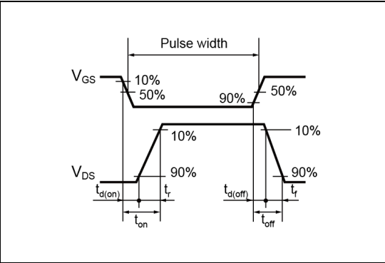
Fig.1-2 Switching Waveforms
