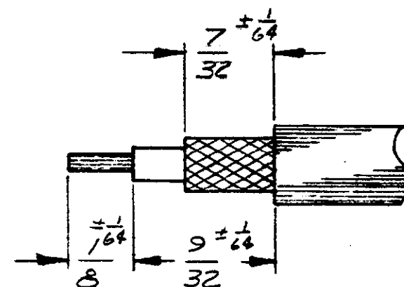
STRIP LENGTH
