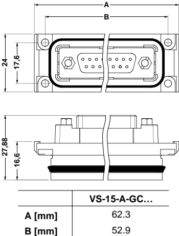
Dimensional drawing: VS-15-A-GC...
