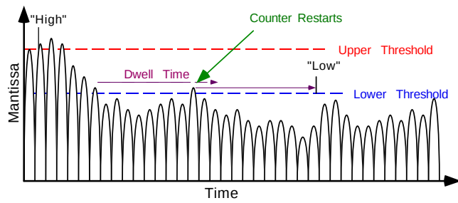
Figure 22. Threshold Settings for IG and DG
