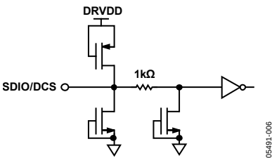
Figure 5x. Equivalent SDIO/DCS Input Circuit
