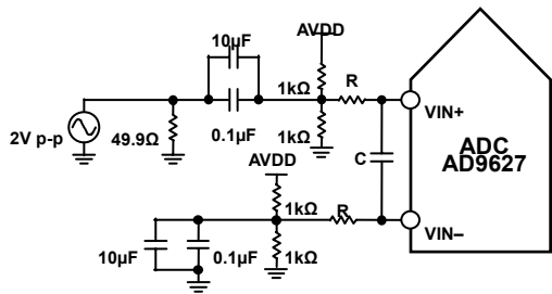
Figure 8 details a typical single-ended input configuration.
