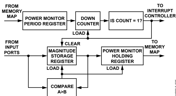
Figure 23. ADC Input Peak Detector Block Diagram
