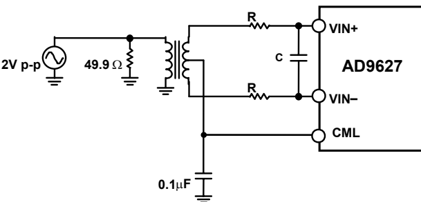
Figure 5. Differential Transformer-Coupled Configuration
