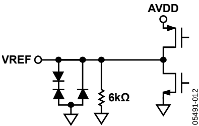
Figure 9. Equivalent VREF Circuit
