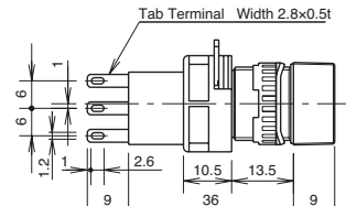
Solder/Tab Terminal
