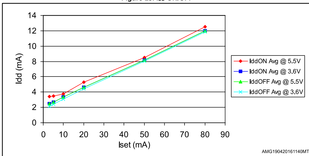
Figure 13: I_{DD} ON/OFF
