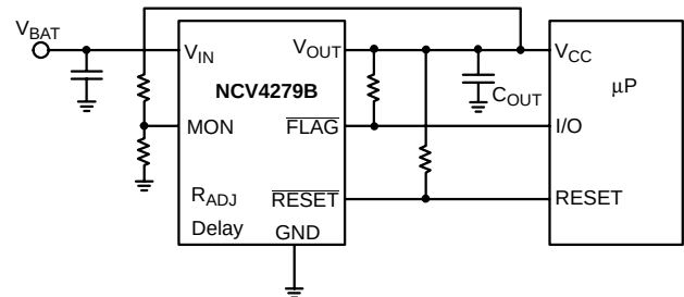
Figure 13. \overline{\text{FLAG}} /Monitor Function
