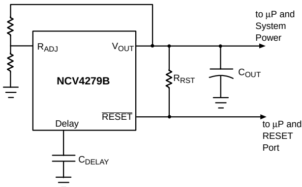
Figure 12. Adjustable \overline{\text{RESET}}
