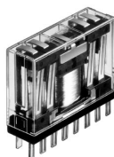
4C 2 coil latching (NC4D-L2)
