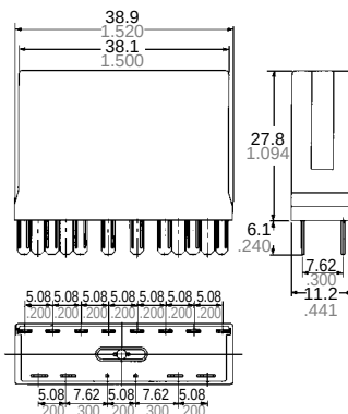
Amber sealed type
