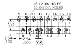
PC board pattern (Copper-side view)
