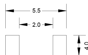
Recommended Solder Pad Layout
