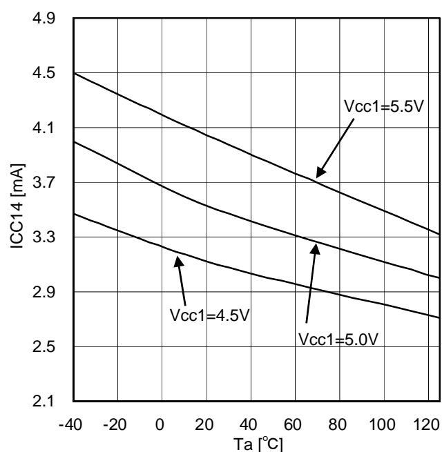
Figure 24. Input side circuit current (at INA=20\text{kHz} and Duty=50\% )
