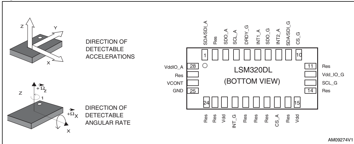
Figure 2. Pin connection
