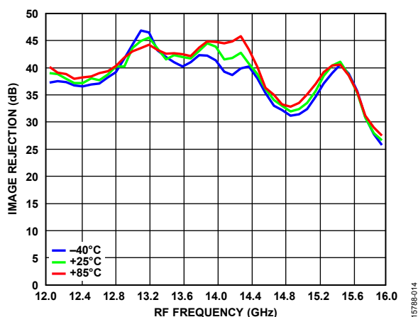
Figure 14. Image Rejection vs. RF Frequency at Various Temperatures
