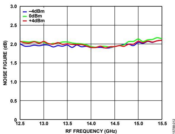
Figure 12. Noise Figure vs. RF Frequency at Various LO Powers
