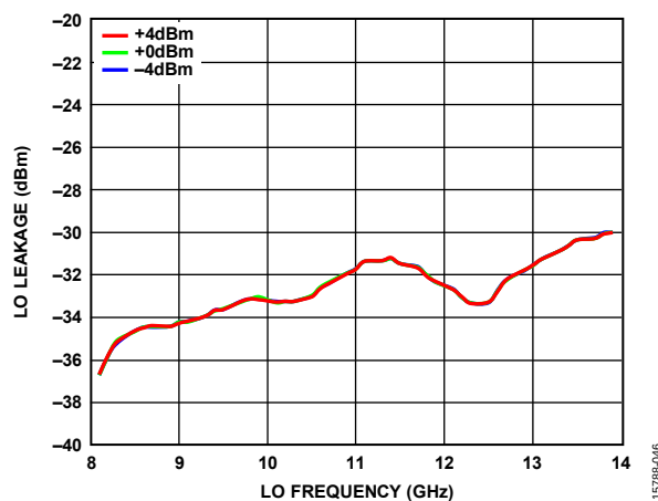
Figure 39. LO Leakage at RFIN vs. LO Frequency at Various LO Powers
