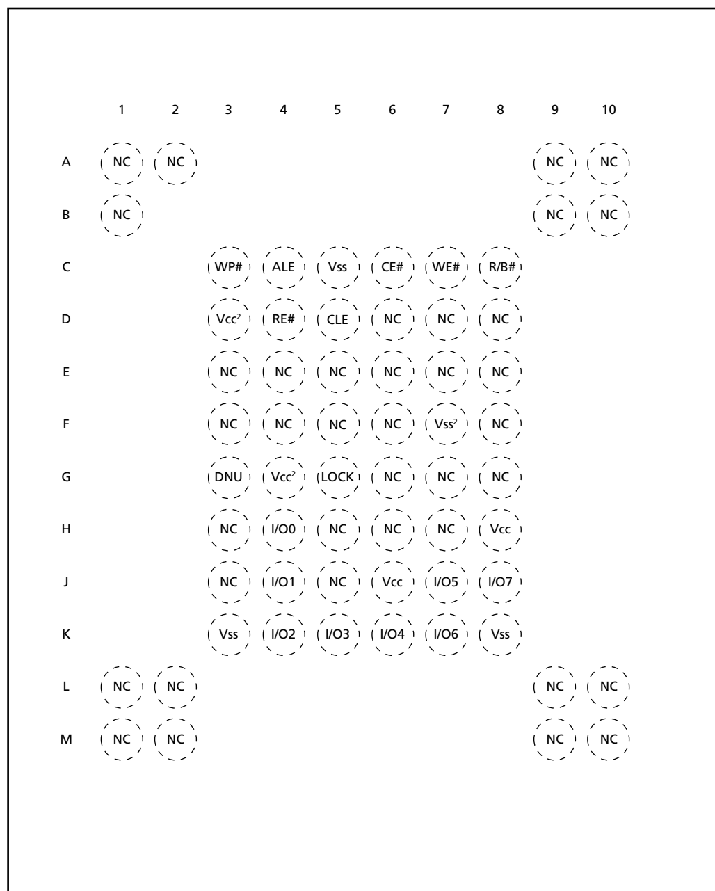
Figure 5: Ball Assignment: 63-Ball VFBGA (x8)
