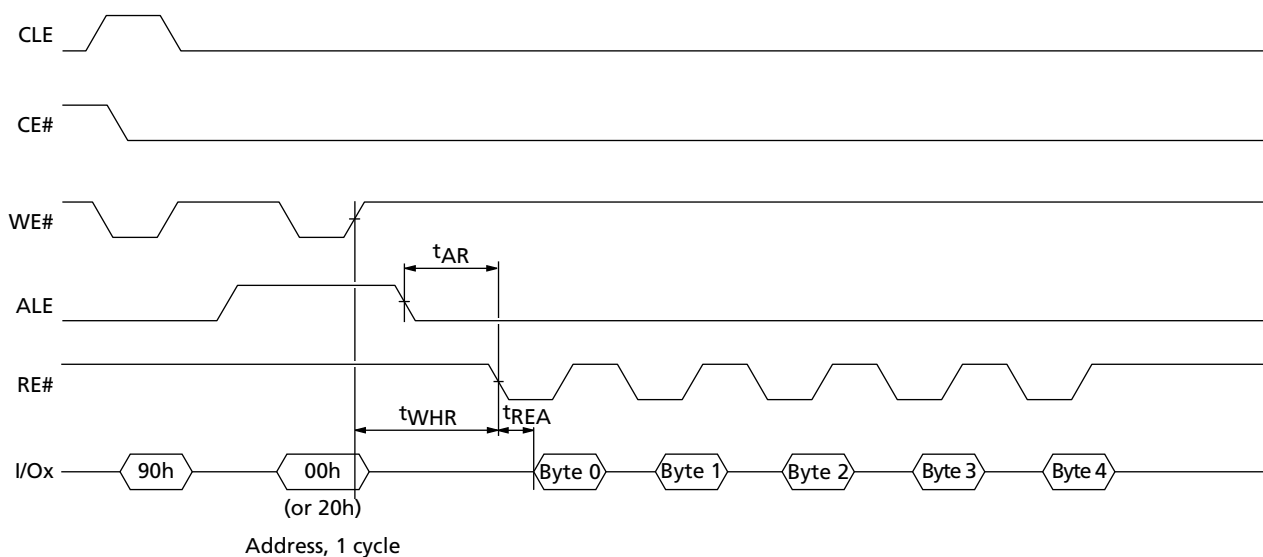
Figure 67: READ ID Operation
