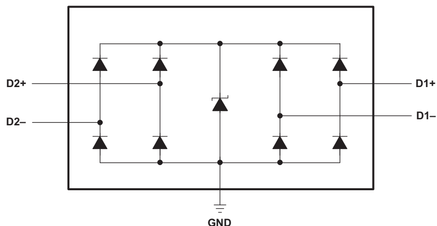
Figure 7. TPD4S010
