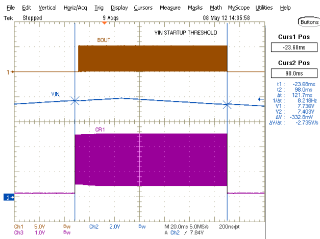
Figure 5 - VIN Startup Threshold
