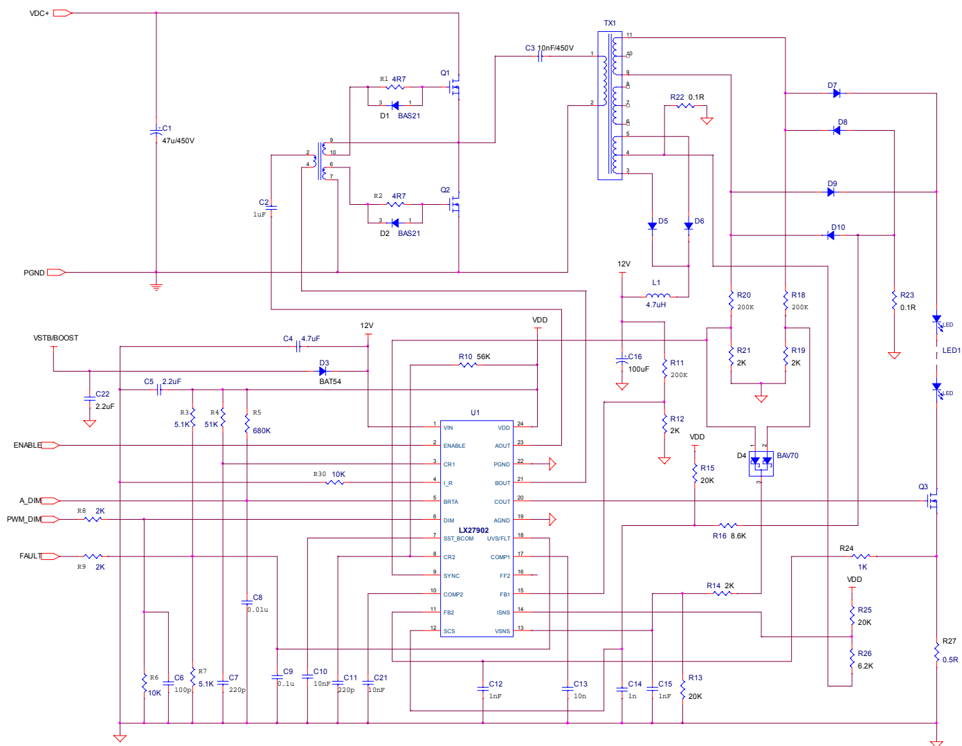
Figure 27 - Application Schematic
