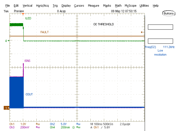
Figure 20 • OC Threshold
