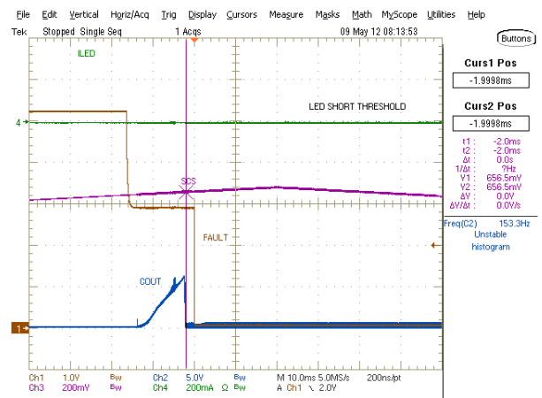
Figure 22 - LED Short Threshold
