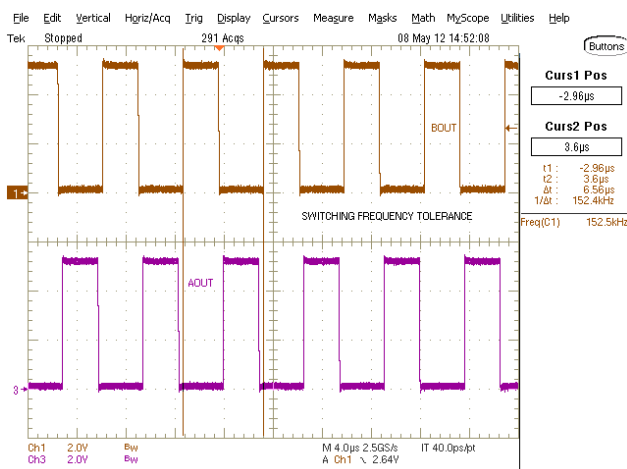
Figure 7 - Switching Frequency Tolerance
