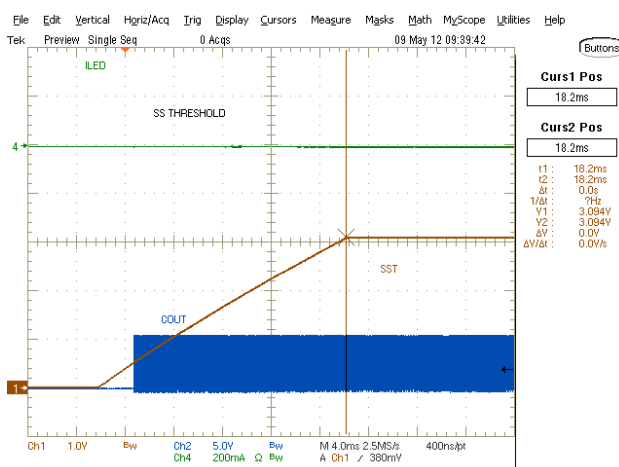
Figure 25 - SS Threshold
