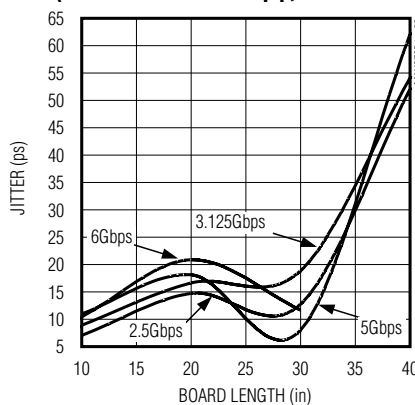
DETERMINISTIC JITTER vs. BOARD LENGTH (FR-4) (INPUT LEVEL OF 500mV p-p , TEST PATTERN)
