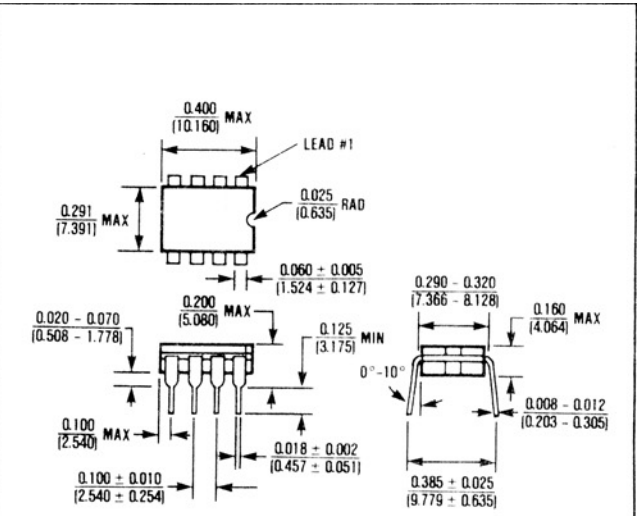
8 Lead Cerdip (JA) \theta_{JA} = 125^{\circ}\text{C/W} \theta_{JC} = 55^{\circ}\text{C/W}
