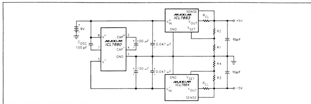
Figure 7. ±5V power supply using one 9V battery.
