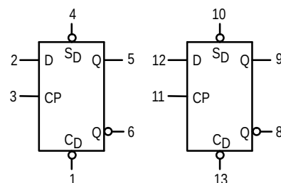
LOGIC SYMBOL
