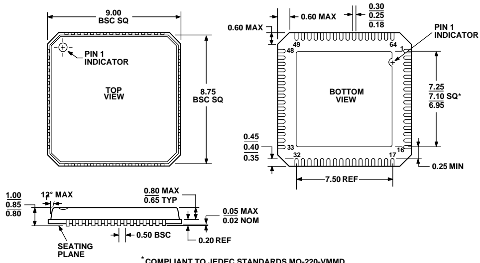
Figure 87. 64-Lead Lead Frame Chip Scale Package (LFCSFP) [CP-64]
