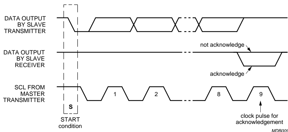
Fig.9 Acknowledge on the I 2 C-bus.
