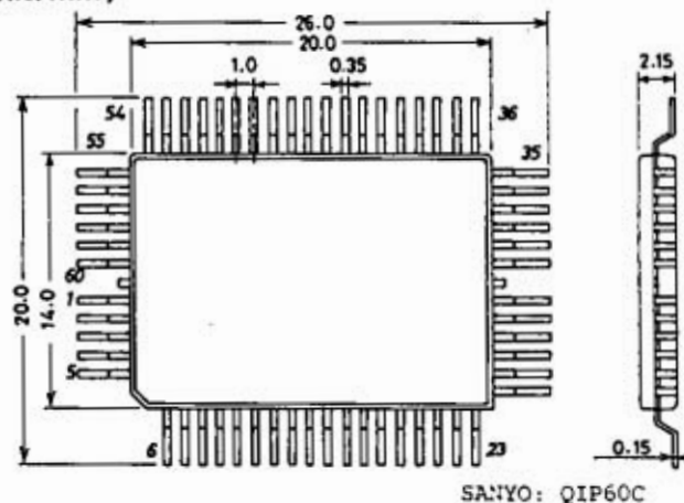
Package Dimensions 3055A-Q60C1C (unit: mm)
