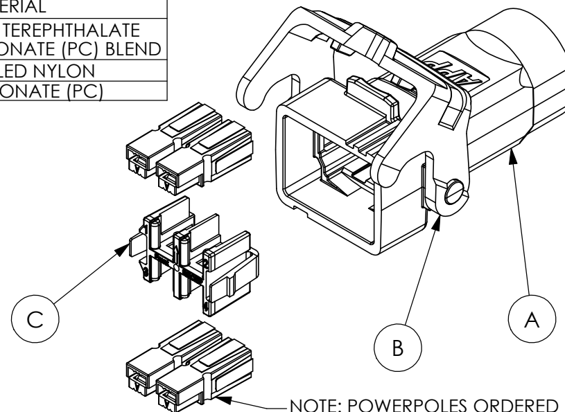
IN-LINE RECEPTACLE MATED WITH PLUG WITH LATCH
