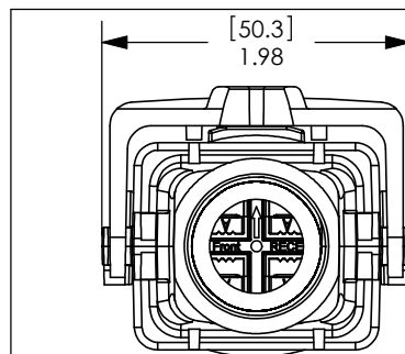
IN-LINE RECEPTACLE MATED WITH PLUG WITH LATCH
