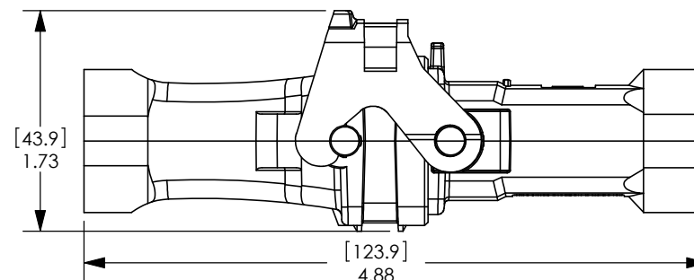
IN-LINE RECEPTACLE MATED WITH PLUG WITH LATCH
