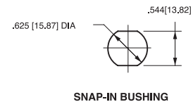
SNAP-IN BUSHING
