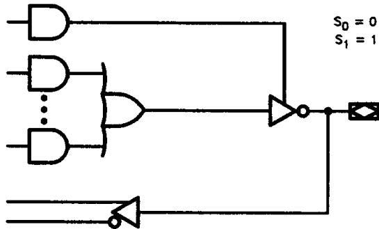
FIGURE 3-3. Combinatorial/Active Low
