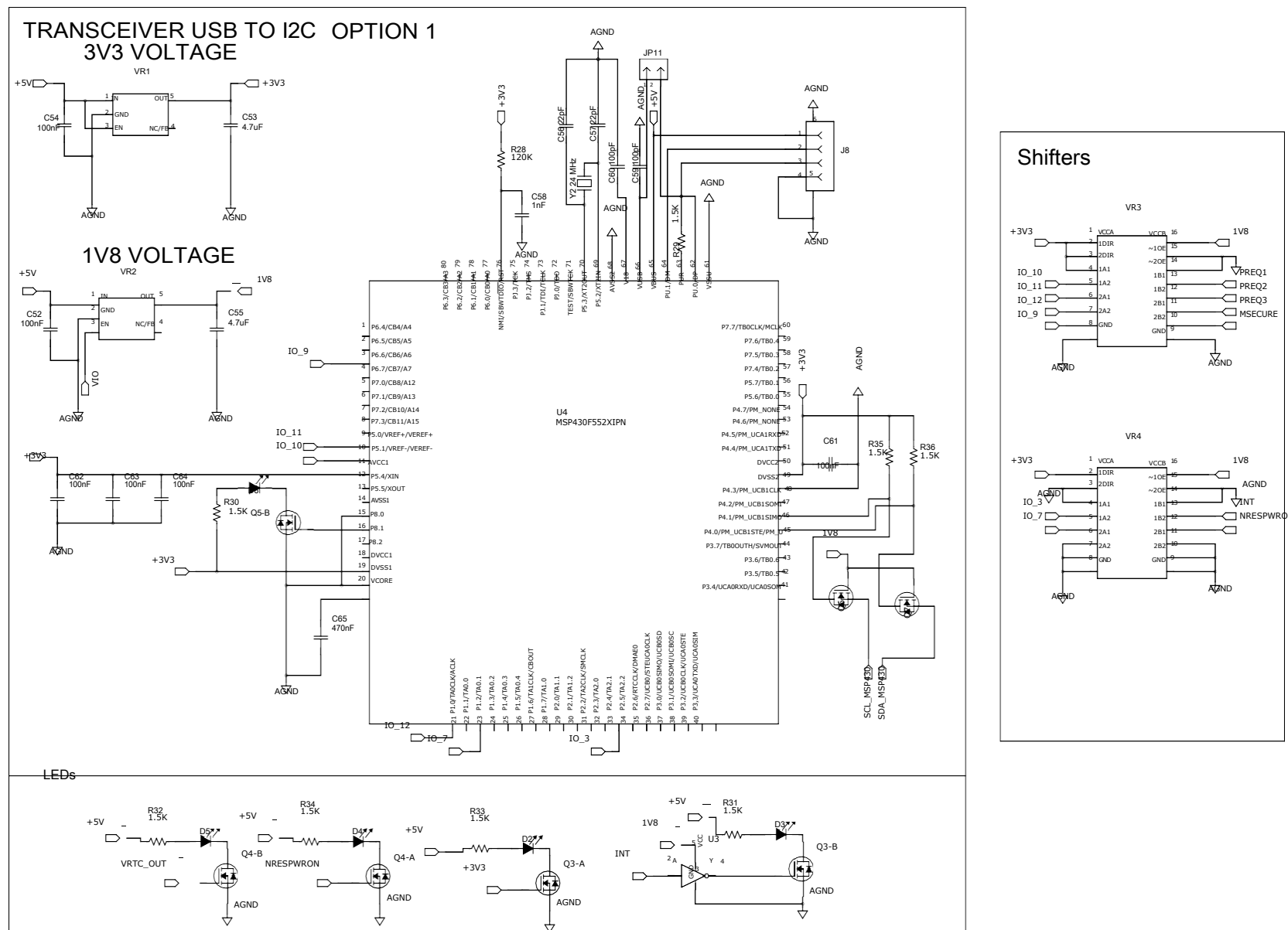
Figure 3. TWL6032 EVM Schematic – MSP430 Connections
