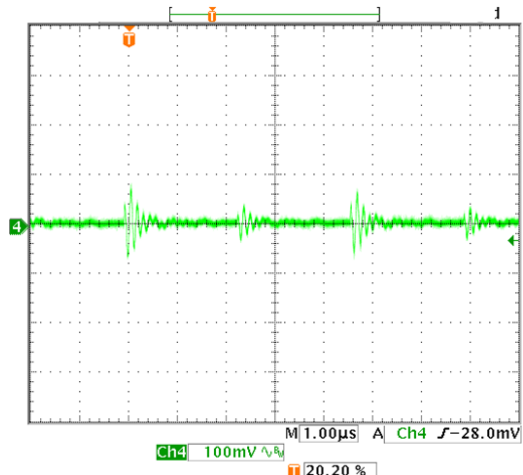
Output Ripple and Noise ( V_{in}=48\text{V} , V_{out}=\text{nom} , I_{out}=0\text{A} , C_{load}=1\mu\text{F} , T_a=+25^\circ\text{C} )
