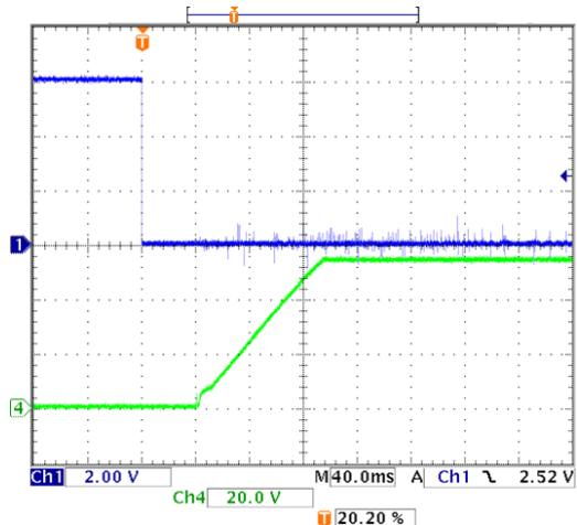
On/Off Enable Delay ( V_{in}=48\text{V} , I_{out}=3\text{A} , T_a=+25^\circ\text{C} ) Trace 1=Enable, Trace 4= V_{out} .
