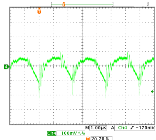
Output Ripple and Noise ( V_{in}=48\text{V} , V_{out}=\text{nom} , I_{out}=3\text{A} , C_{load}=1\mu\text{F} , T_a=+25^\circ\text{C} )
