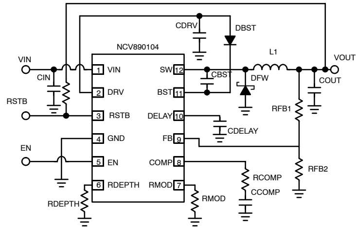
Figure 1. Typical Application
