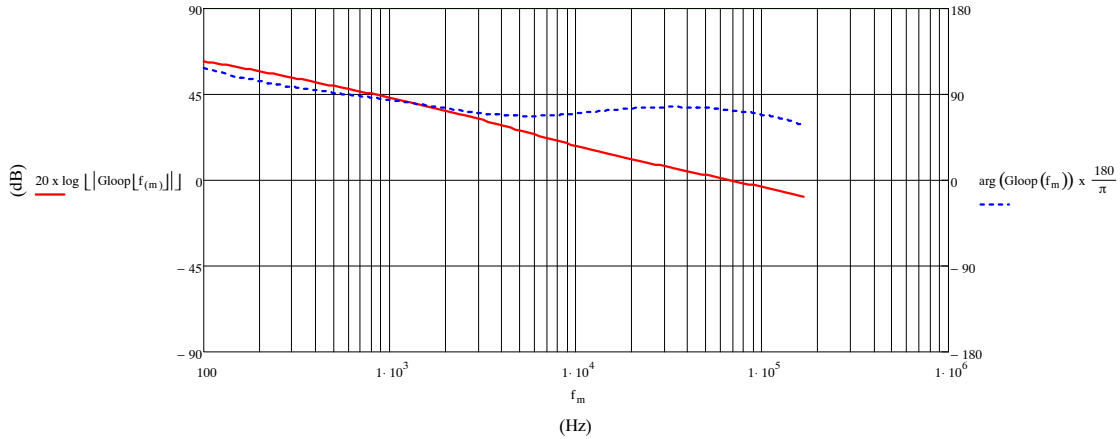
Figure 36. Bode Plot of the Total Loop
