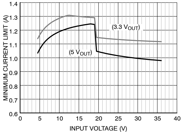
Figure 26. NCV890104 Load Current Capability with 4.7 \mu H Inductor
