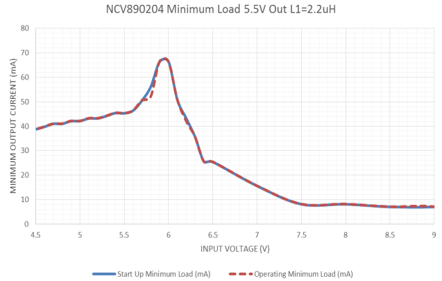
Typical Minimum Load 5.5 V Out, L_1 = 2.2 \mu\text{H}
