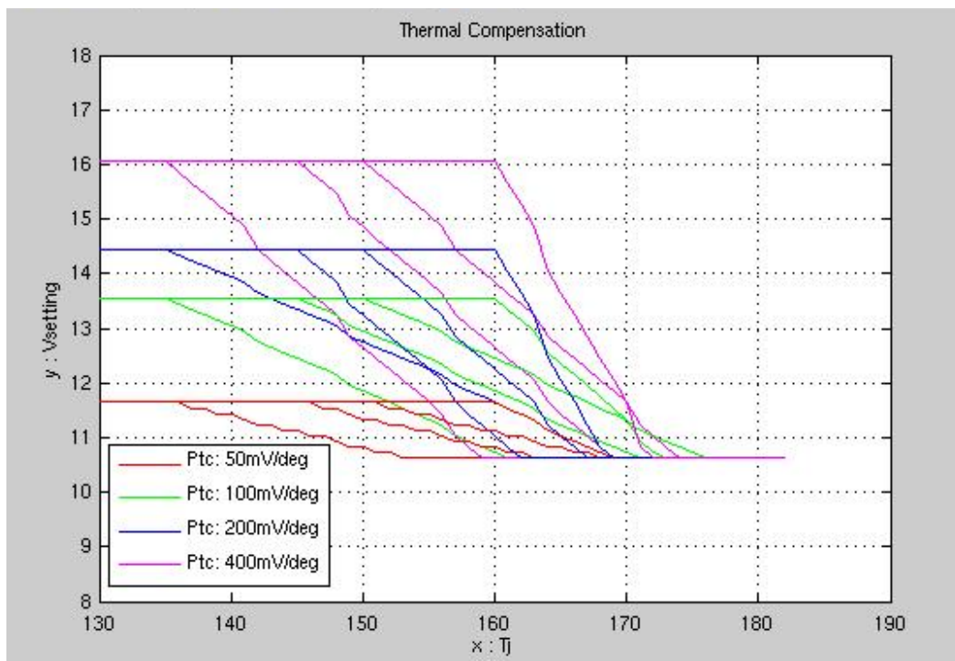
Figure 11. Thermal Compensation
