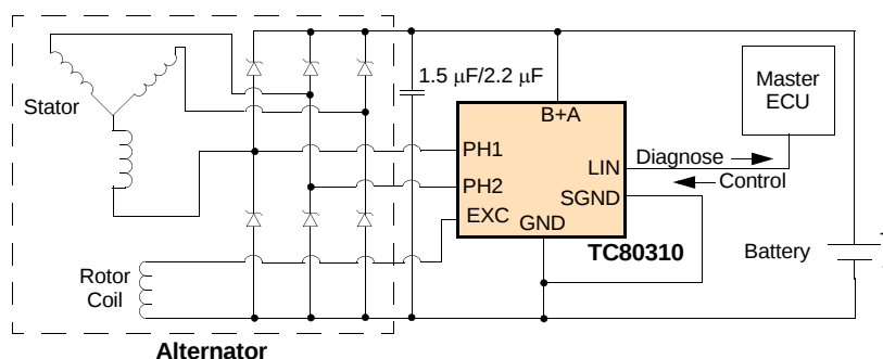
Figure 1. 80310 Simplified Application Diagram (LIN Mode)
