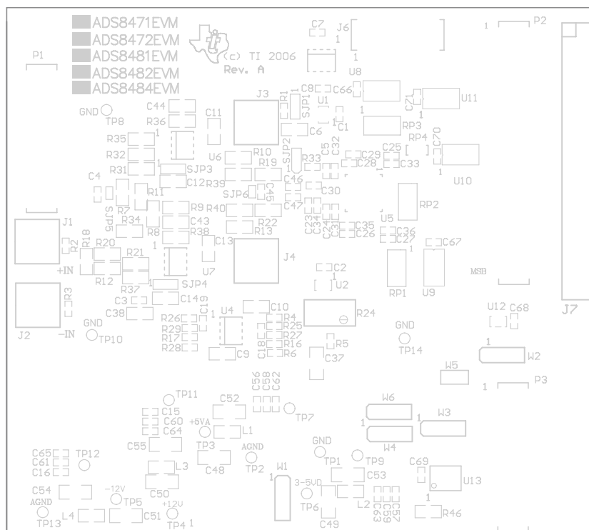
Figure 6. Top Overlay
