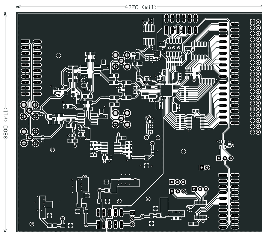
Figure 2. Top – Layer 1
