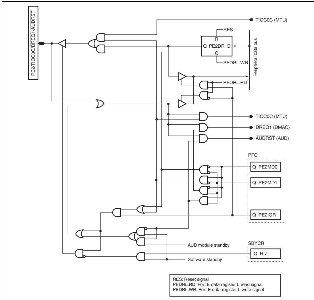
Figure D.48 PE2/TIOC0C/ \overline{\text{DREQ1}} /AUDRST
