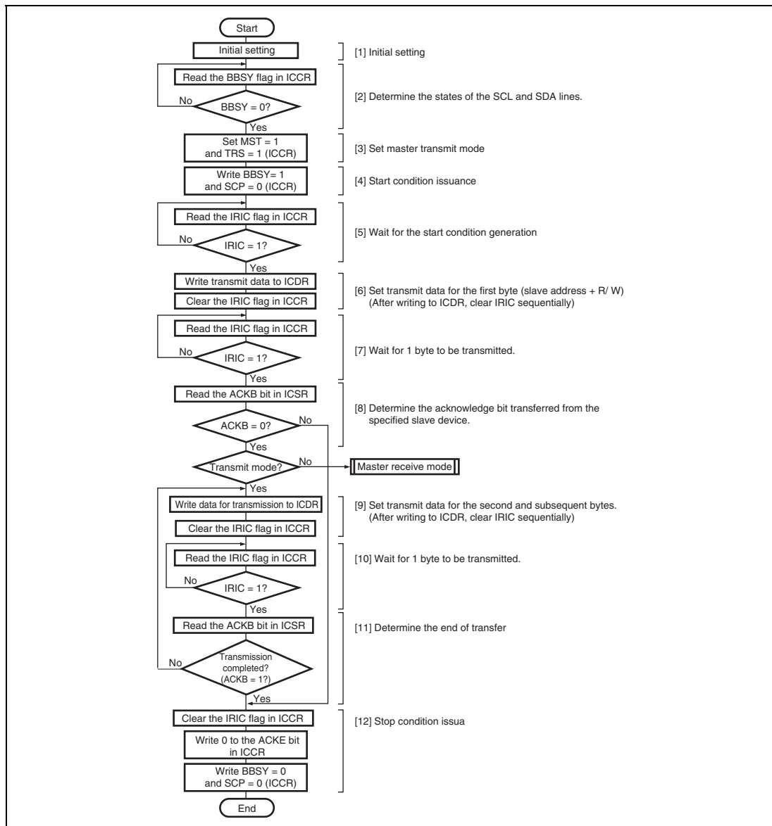
Figure 14.7 Example: Flowchart of Operations in the Master Transmit Mode
