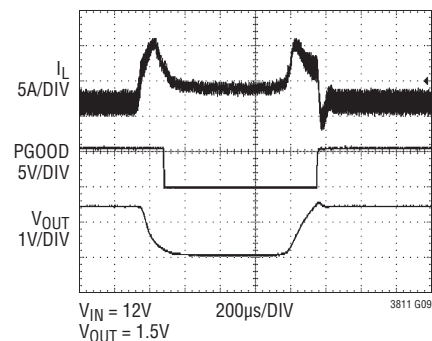
Short-Circuit Waveforms
