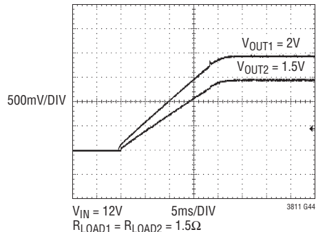
Ratiometric Tracking Start-Up
