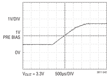
Start-Up Into a Pre-Biased Output Capacitor
