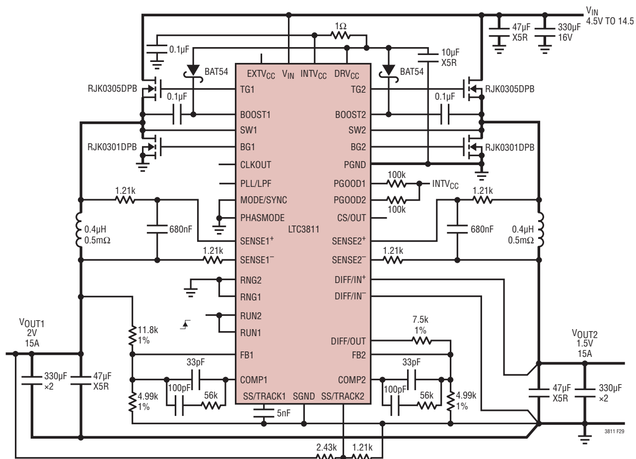
Figure 29. High Efficiency Core-I/O Power Supply with Differential Remote Sensing and Tracking
