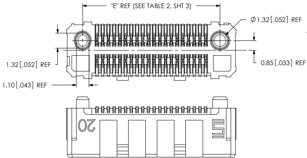
FIG 1 (LSHM-1XX-XX.X-DV-A-N-X-TR SHOWN)
