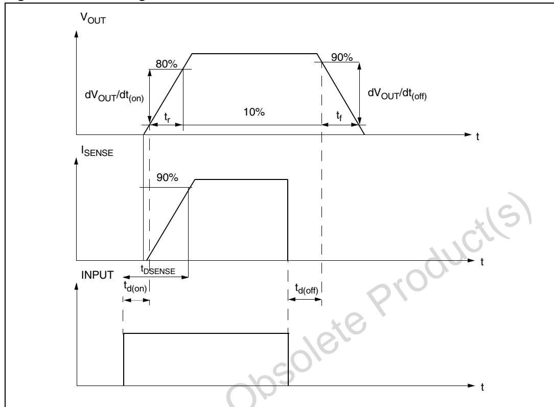
Figure 5. Switching characteristics
