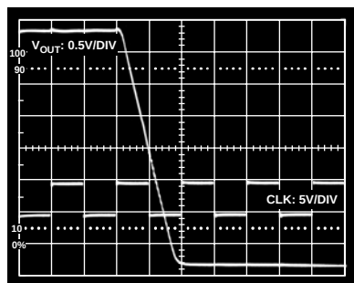
Figure 18. Large Signal Settling (0.5 \mu s/DIV)
