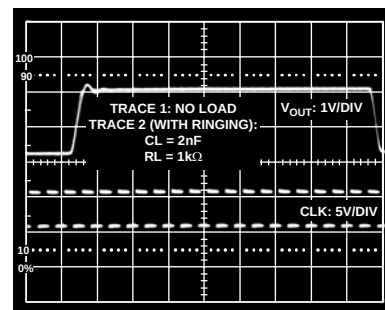
Figure 20. Capacitive Load Output Performance (2 \mu s/DIV)
