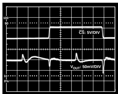
Figure 19. Midscale Glitch and Digital Feedthrough (2 \mu s/DIV)
