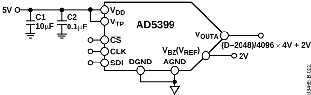
Figure 22. Basic Connection
