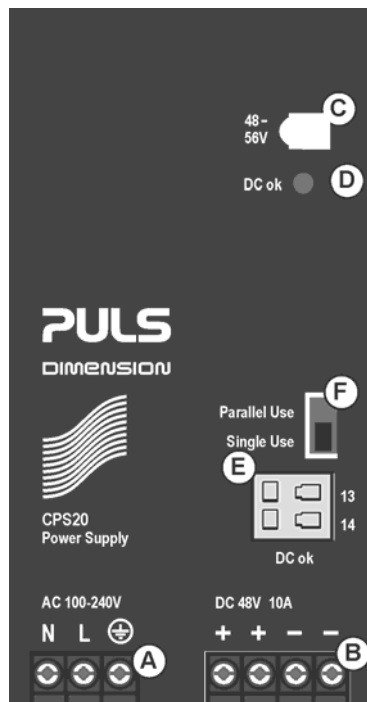
Fig. 13-1 Front side
