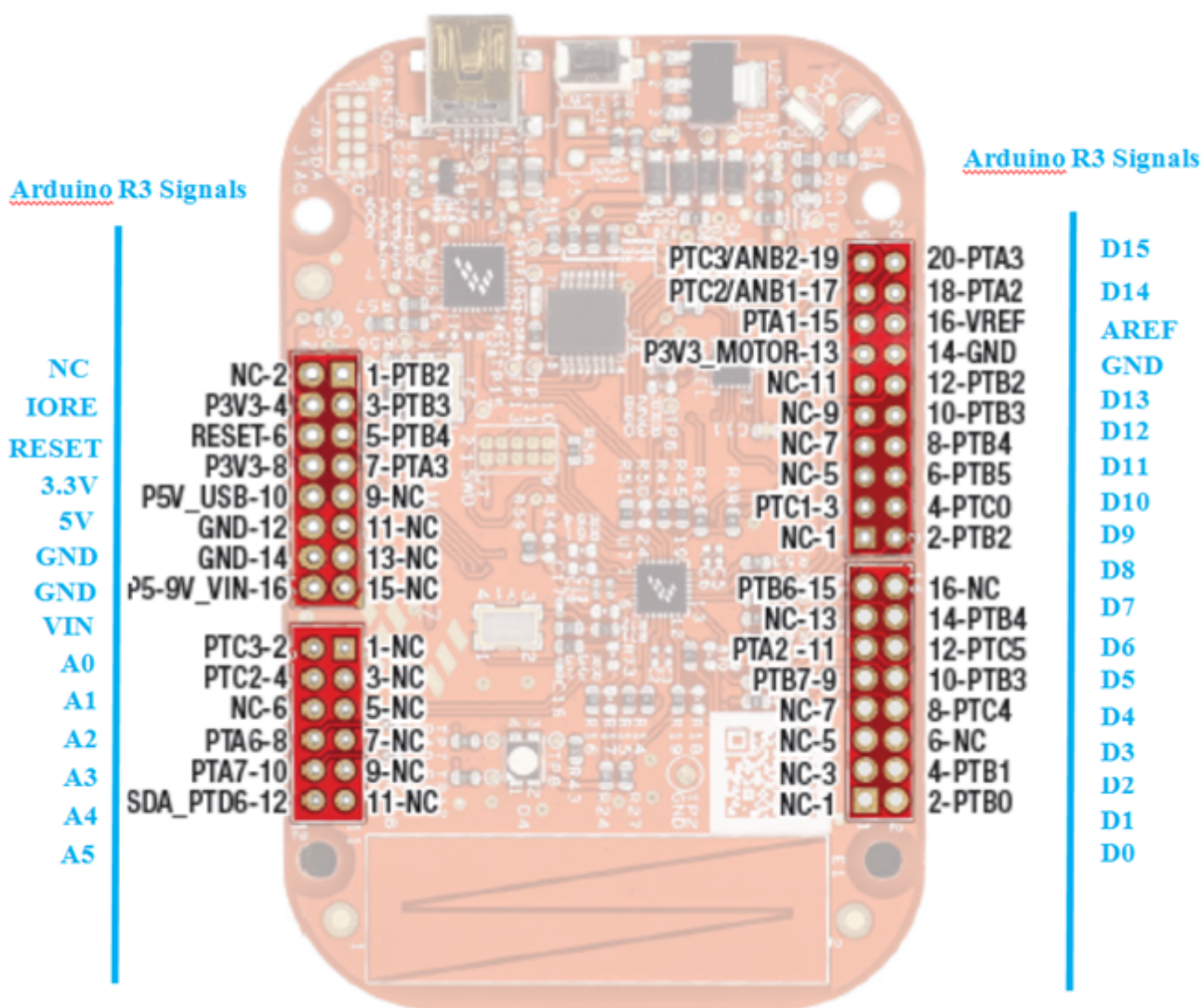
Figure 9. I/O headers
