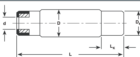
Figure 2: GWK 20...GWK 300
