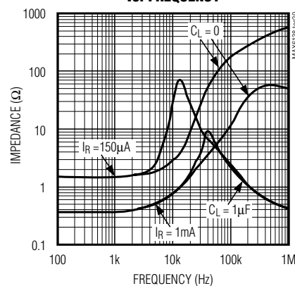
MAX6138_12 OUTPUT IMPEDANCE vs. FREQUENCY
