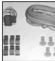
2517F Wishbone 5-Wire Trailer Wiring Kit. 25-FT wishbone style 5-wire to 4-wire trailer harness w/ molded plug. 4-ft. trunk wire harness. 2-wire connectors & 8 frame clips all included. 5th wire allows for utility and running light
