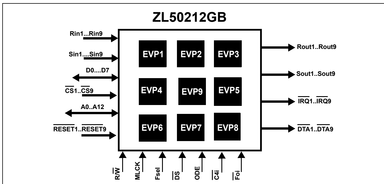
Figure 1 - ZL50212 Device Overview
