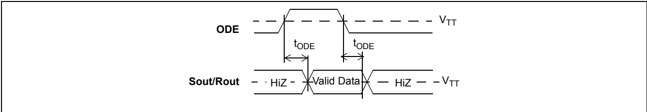
Figure 13 - Output Driver Enable (ODE)
