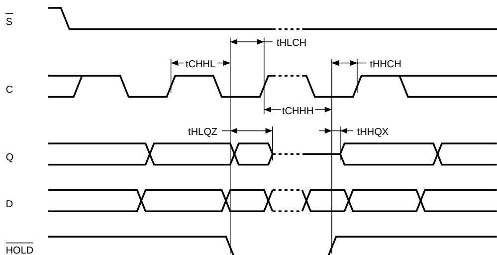
Figure 18. Hold Timing
