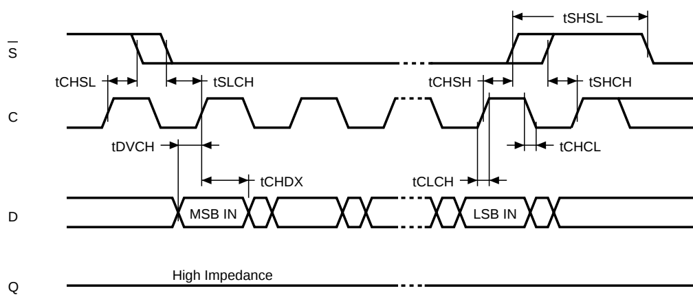
Figure 17. Serial Input Timing
