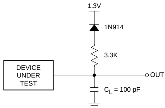
Figure 2. A.C. Testing Load Circuit (example)
